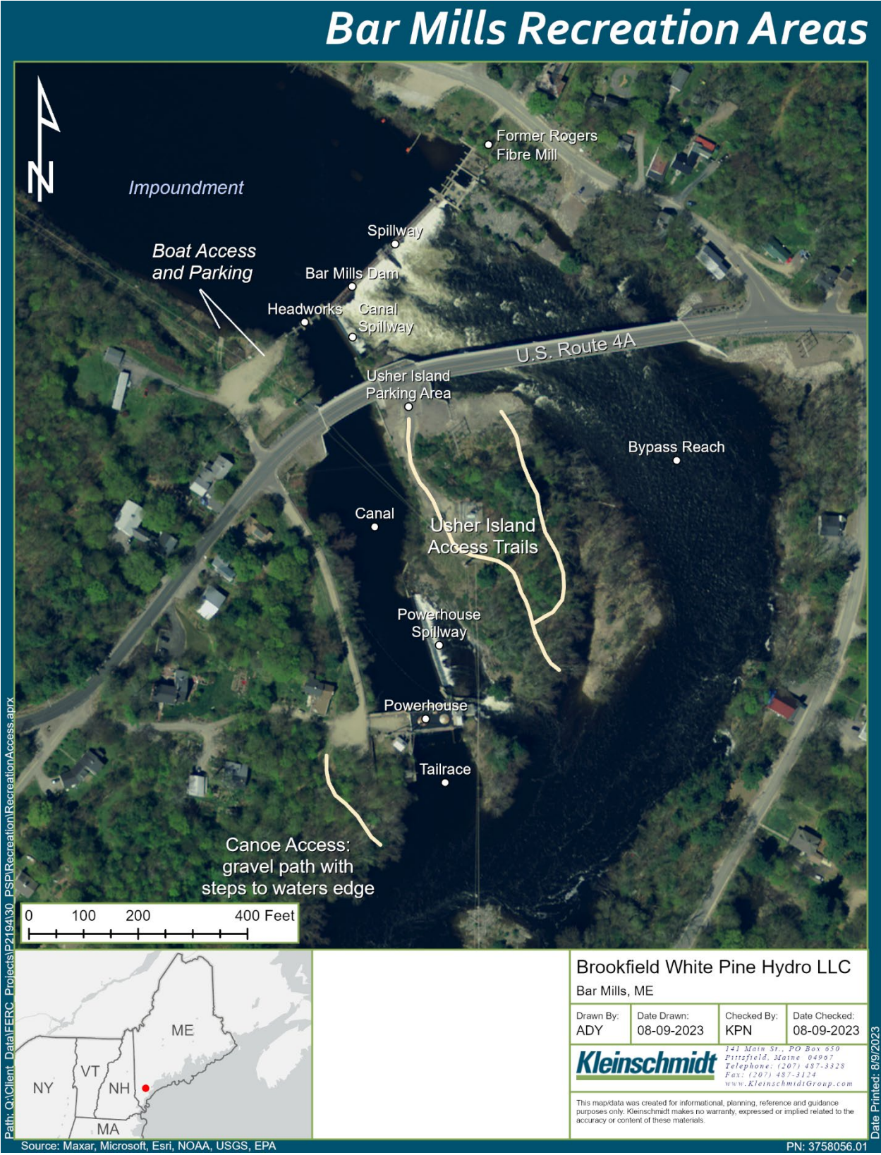
Figure 2 Bar Mills Project Features
